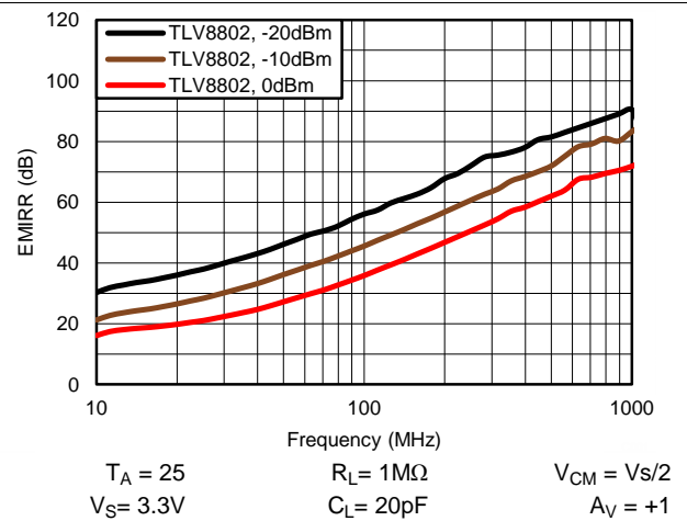
Figure 36. EMIRR Performance
