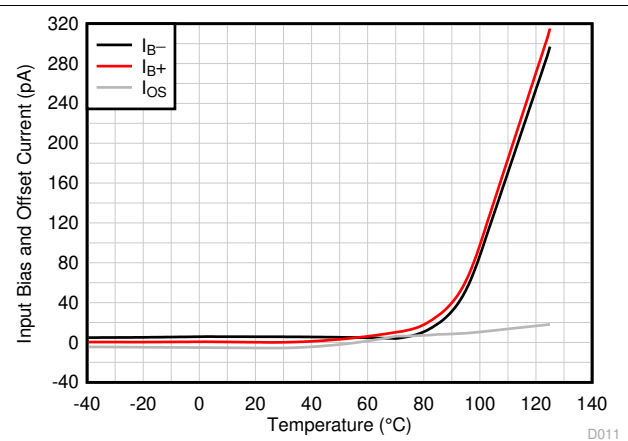
Figure 5-10. Input Bias Current vs Temperature
