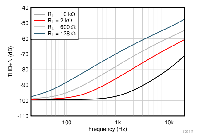
Figure 5-20. THD+N Ratio vs Frequency BW = 80kHz, V_{OUT} = 3.5V_{RMS}
