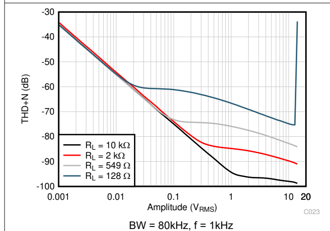
Figure 5-21. THD+N vs Output Amplitude BW = 80kHz, f = 1\text{kHz}
