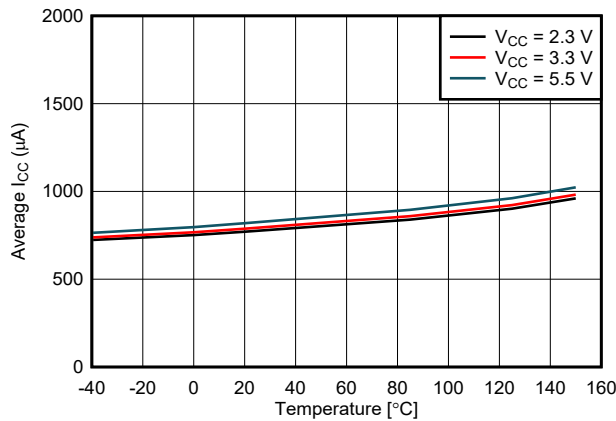
Figure 6-15. Standby Mode Supply Current vs. Temperature
