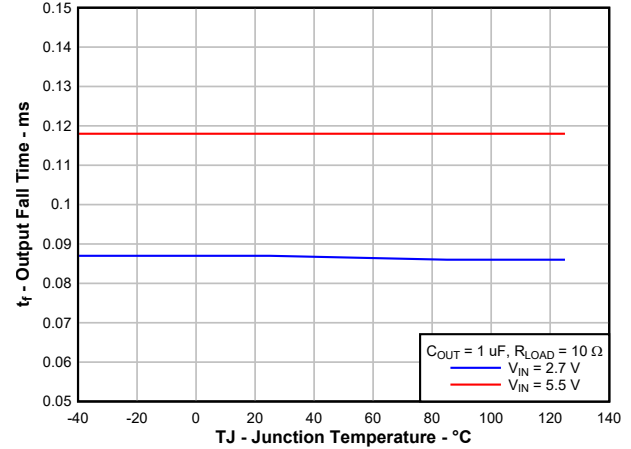
Figure 6-14. Output Fall Time ( T_F ) vs Temperature
