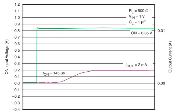
Figure 20. t_{ON} Response
