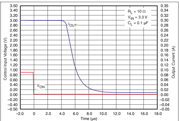
Figure 23. t_{OFF} Response
