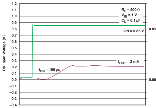
Figure 19. t_{ON} Response
