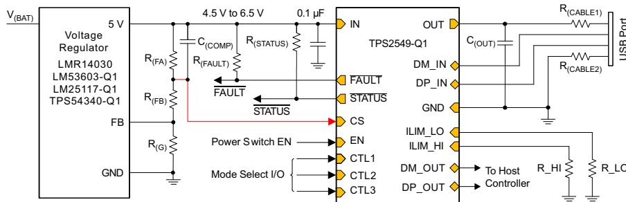
Simplified Schematic
