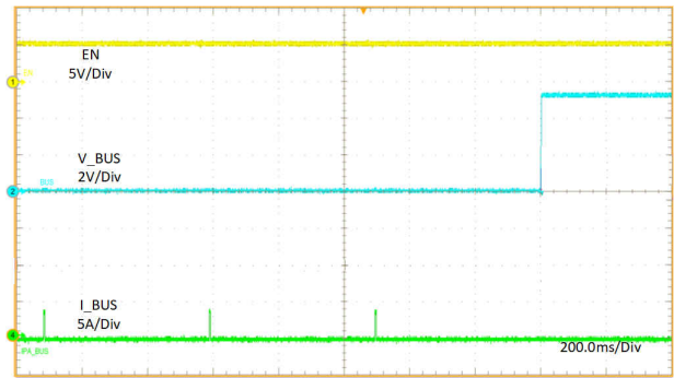
A. EN is High BUS removed from GND
