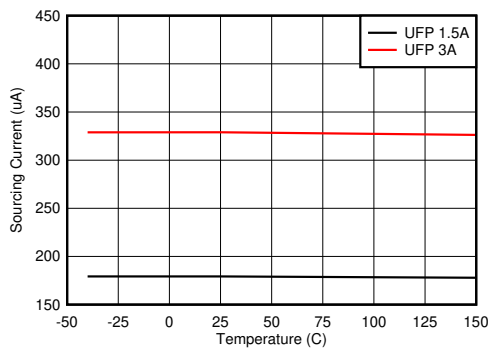
Figure 8-21. CC Sourcing Current vs Junction Temperature
