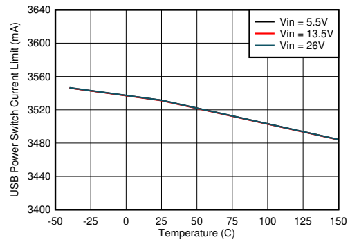
Figure 8-10. USB Power Switch Current Limit vs Junction Temperature ILIM = GND
