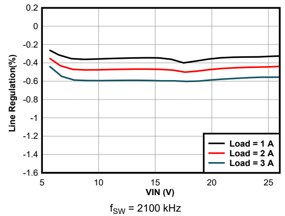
Figure 11-7. Line Regulation
