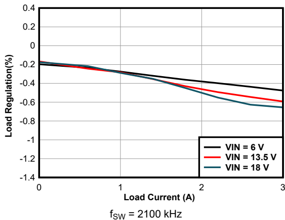
Figure 11-6. Load Regulation
