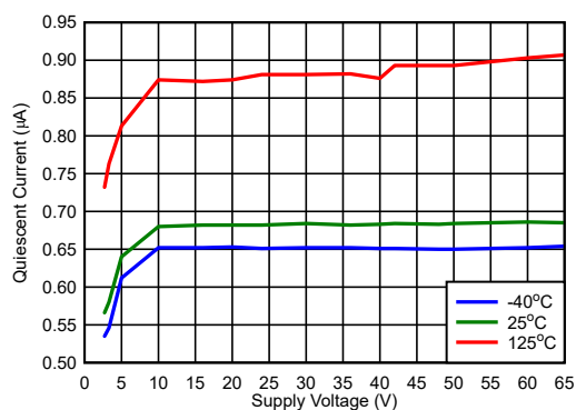
Typical I_{DD} vs V_{DD}
