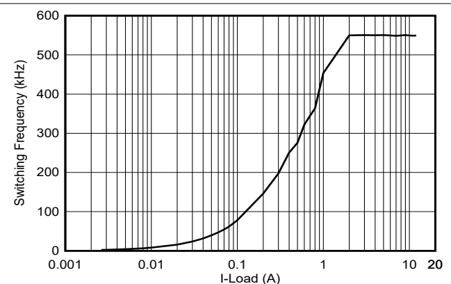
Figure 7-7. Switching Frequency vs Output Load (ECO)
