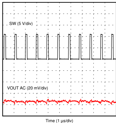
Figure 7-26. Output Voltage Ripple
