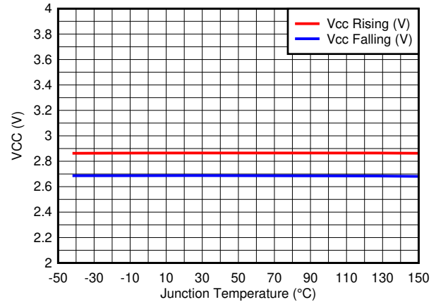
Figure 5-8. VCC UVLO
