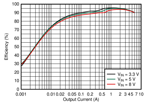
Figure 7-5. Efficiency – 1100 kHz, FCCM, External 3.3-V VCC, 0-Ω R_{BOOT}
