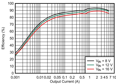
Figure 7-4. Efficiency – 1100 kHz, FCCM, External 3.3-V VCC, 4.7-Ω R_{BOOT}
