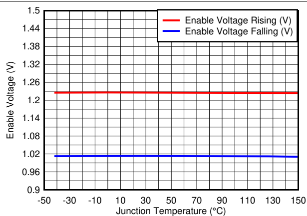
Figure 5-5. Enable Voltage
