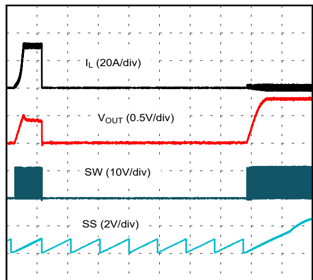
Figure 6-2. Exiting Hiccup
