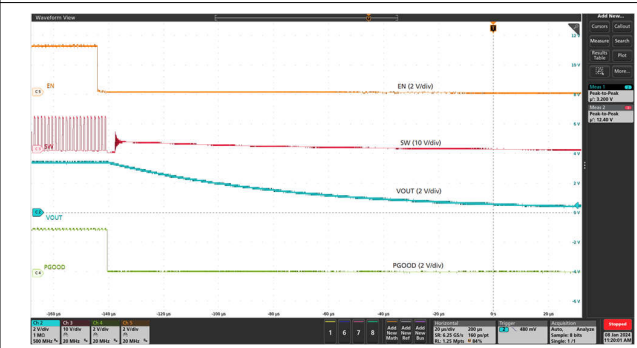
V_{IN} = 12V V_{OUT} = 3.3V I_{OUT} = 25A Figure 7-11. Shutdown With EN
