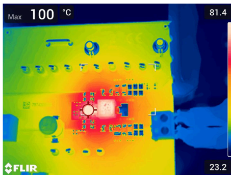
Figure 5-7. Thermal Image – 5V Output, TPS54KB20EVM, 6 Layers
