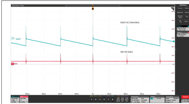
V_{IN} = 12V V_{OUT} = 3.3V I_{OUT} = 10mA Figure 7-8. Output Voltage Ripple – Skip-mode
