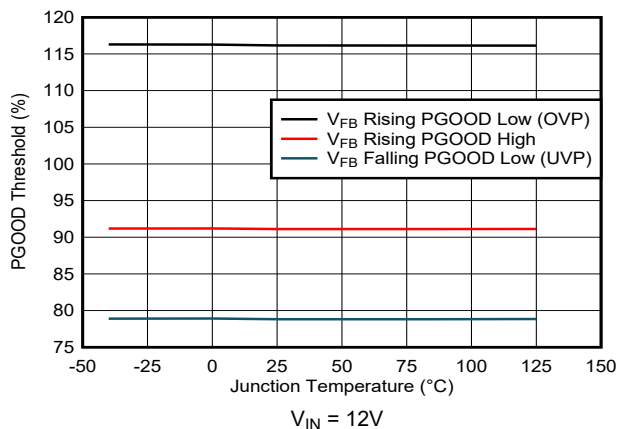
Figure 5-35. Power-Good Thresholds versus Junction Temperature (V REF = 0.5V)
