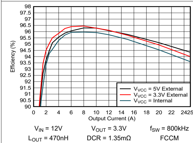
Figure 5-5. Efficiency versus VCC Bias With V_{OUT} = 3.3V
