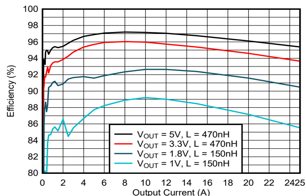
Typical Application Efficiency ( V_{IN} = 12V , f_{SW} = 800kHz , Internal VCC, Skip-Mode)
