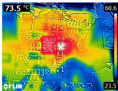
Figure 5-9. Thermal Image – 5V Output, 3 Inch x 3 Inch, 4 Layers
