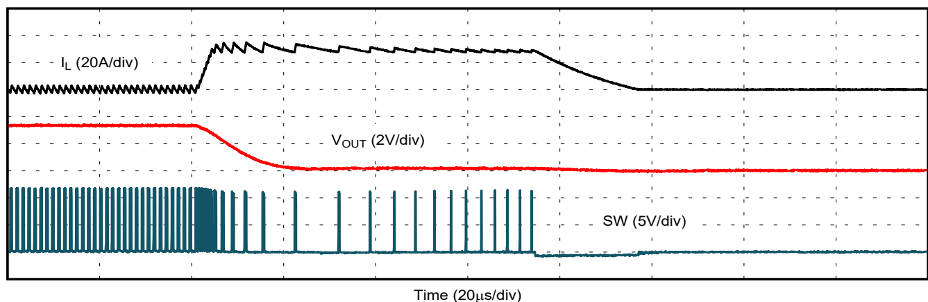
Figure 6-7. Overcurrent Protection
