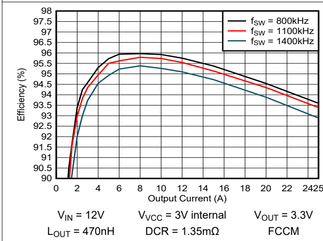
Figure 5-3. Efficiency versus f_{SW} With V_{OUT} = 3.3V
