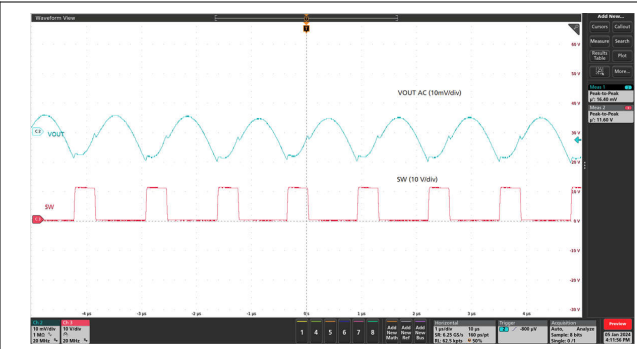
V_{IN} = 12V V_{OUT} = 3.3V I_{OUT} = 25A Figure 7-9. Output Voltage Ripple – FCCM
