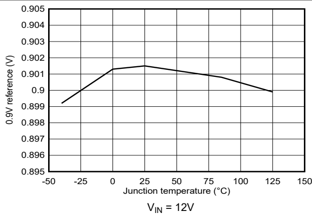
Figure 5-21. 0.9V Reference Voltage versus Junction Temperature
