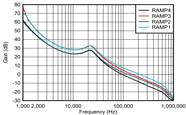
Figure 6-3. Gain versus Ramp Setting - VREF = 0.9V
