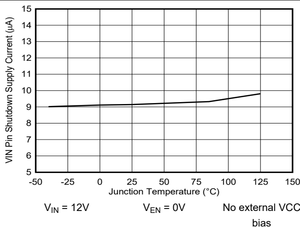
Figure 5-23. VIN Pin Shutdown Quiescent Current versus Junction Temperature
