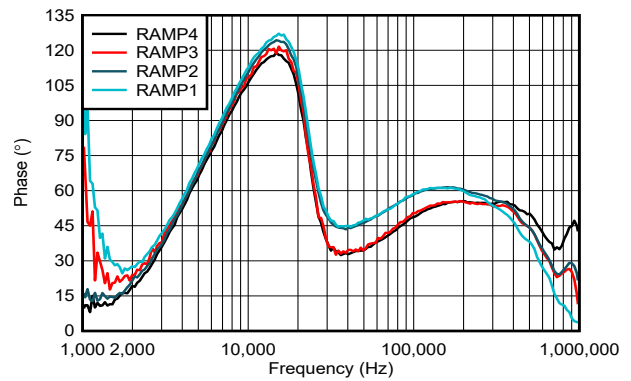
Figure 6-4. Phase versus Ramp Setting - VREF = 0.9V
