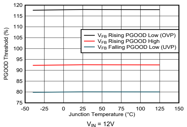
Figure 5-36. Power-Good Thresholds versus Junction Temperature (V REF = 0.9V)
