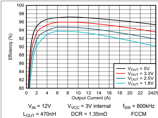
Figure 5-1. Efficiency With V_{OUT} \geq 1.8V
