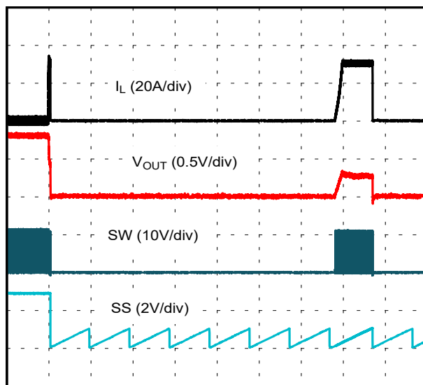
Figure 6-1. Entering Hiccup
