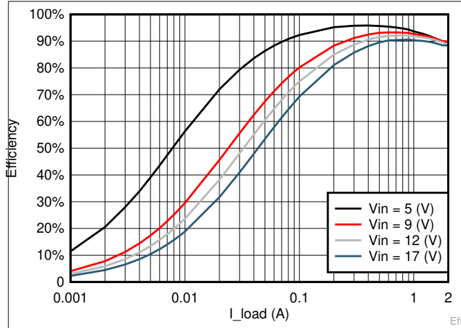
Figure 6-13. V OUT = 3.3 V Efficiency, L = 3.3 μH
