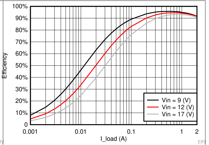
Figure 6-14. V OUT = 5 V Efficiency, L = 4.7 μH
