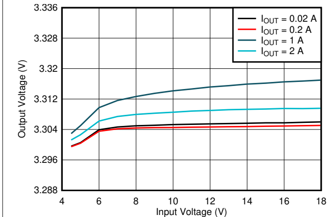
Figure 8-4. Line Regulation
