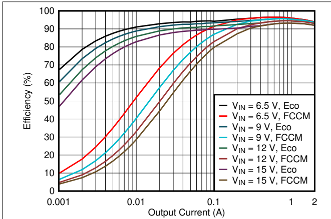
Figure 8-2. Efficiency
