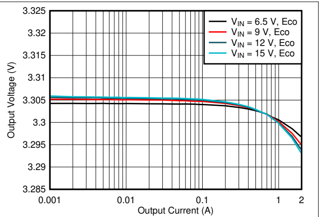
Figure 8-3. Load Regulation
