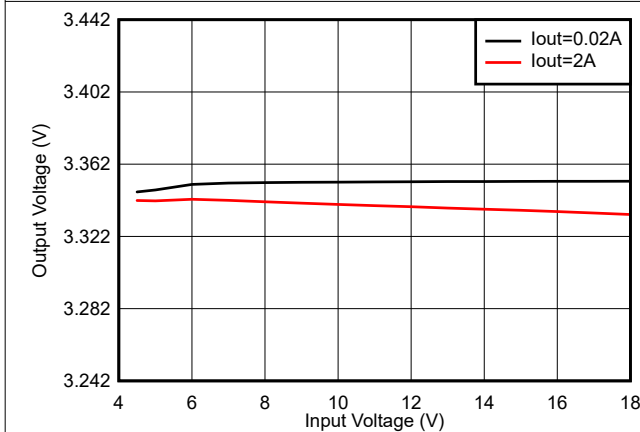
Figure 8-4. Line Regulation
