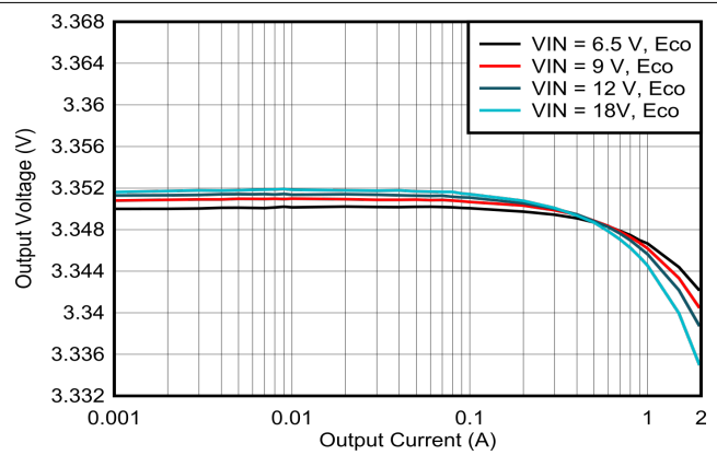
Figure 8-3. Load Regulation
