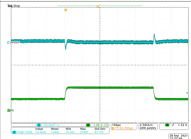
Figure 8-11. Transient Response 1 to 2 A with Slew Rate of 2.5 \text{A}/\mu\text{s}
