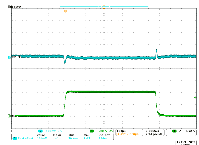
Figure 8-13. Transient Response 0 to 2 A with Slew Rate of 2.5 \text{A}/\mu\text{s} (FCCM)
