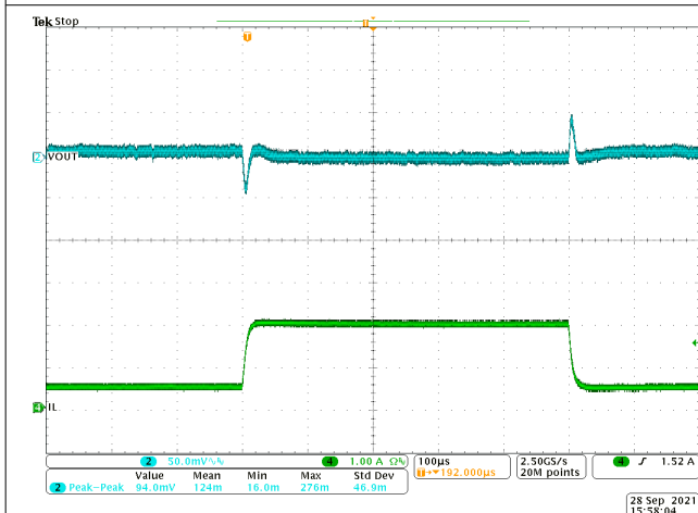
Figure 8-10. Transient Response 0.5 to 2 A with Slew Rate of 2.5 \text{A}/\mu\text{s}
