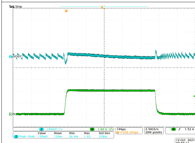
Figure 8-12. Transient Response 0 to 2 A with Slew Rate of 2.5 \text{A}/\mu\text{s} (ECO)
