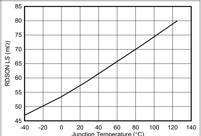
Figure 5-6. High-Side Rdson
