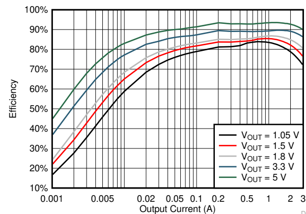
TPS563201 Efficiency
