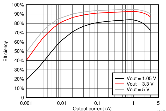
TPS563202 Efficiency
