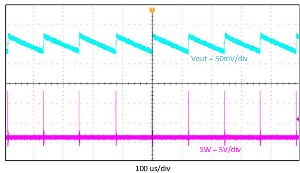
Figure 9-5. Output Voltage Ripple, 10 mA
