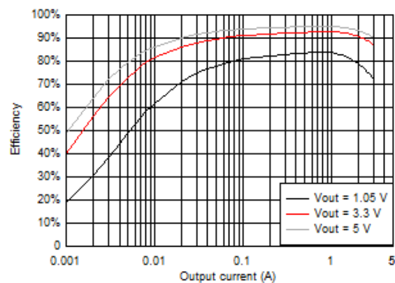
TPS563202S Efficiency
