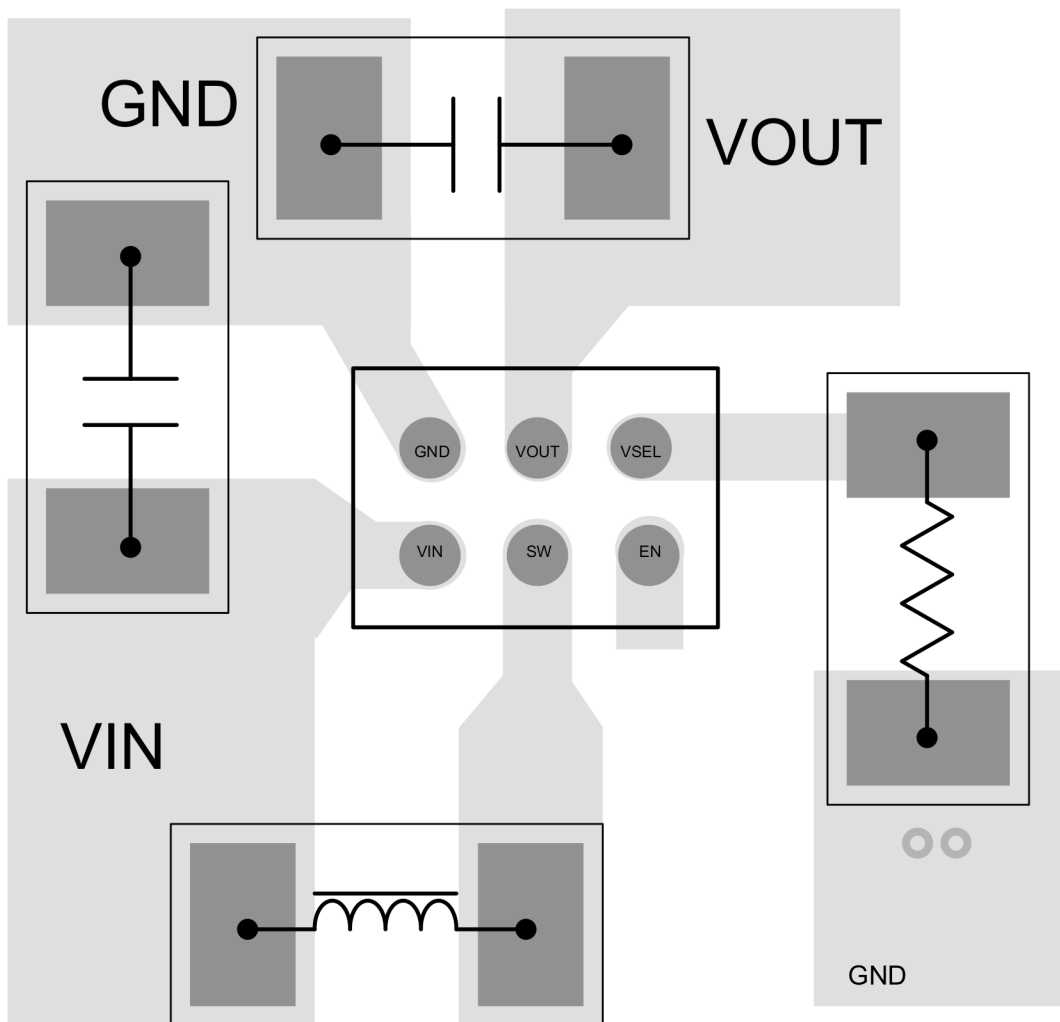
Figure 8-28. Layout Example-YBH
