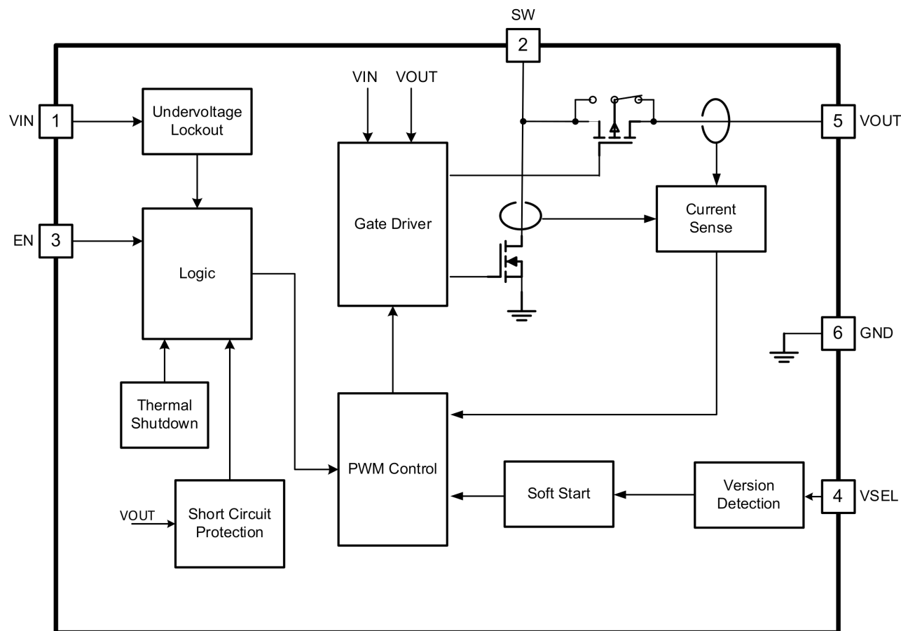
Figure 7-1. Functional Block Diagram
