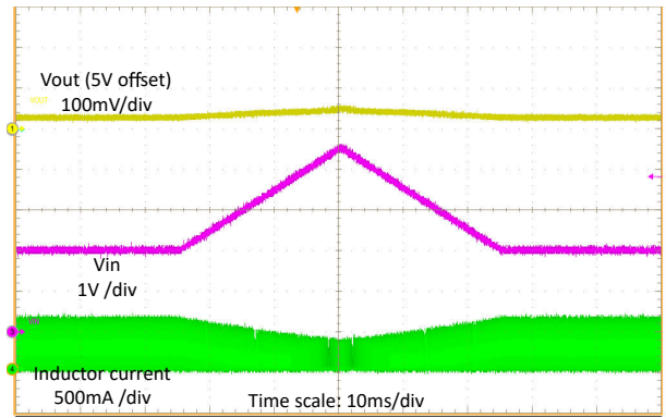
Figure 8-11. Line Sweep
