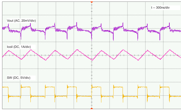
Figure 9-8. PWM Operation, Load = 3 A
