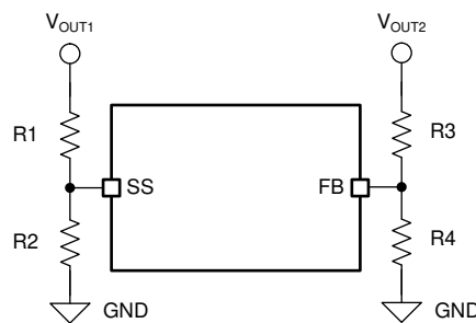
Figure 7-1. Output Voltage Tracking
