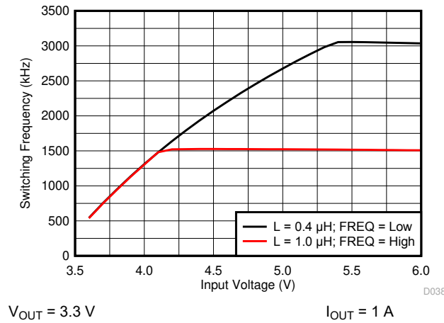
Figure 6-11. Frequency vs Input Voltage
