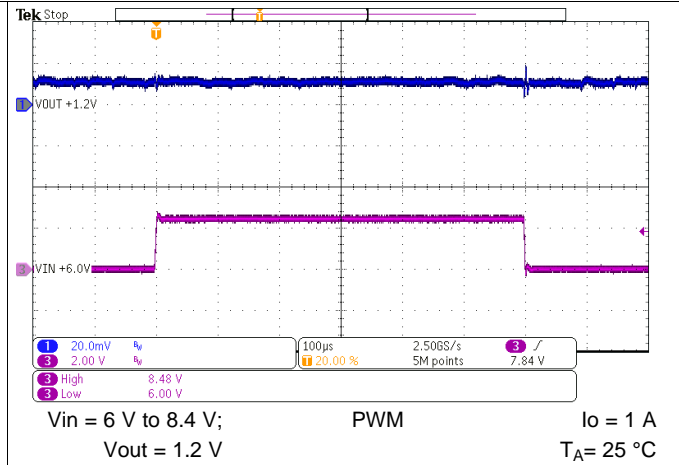
Figure 39. Line Transient Response
