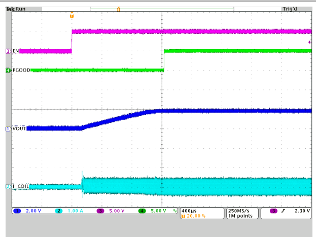
TPS62824A/5A/6A/7A
