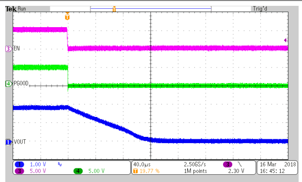
TPS6282x
