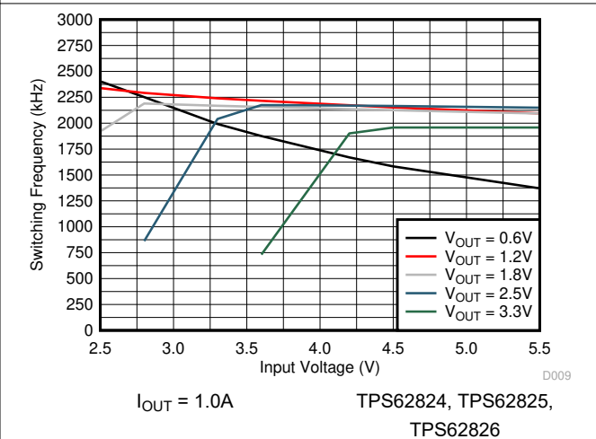
Figure 8-24. Switching Frequency
