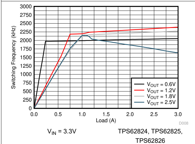
Figure 8-23. Switching Frequency
