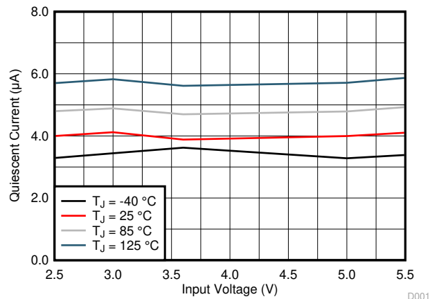
Figure 6-4. Quiescent Current
