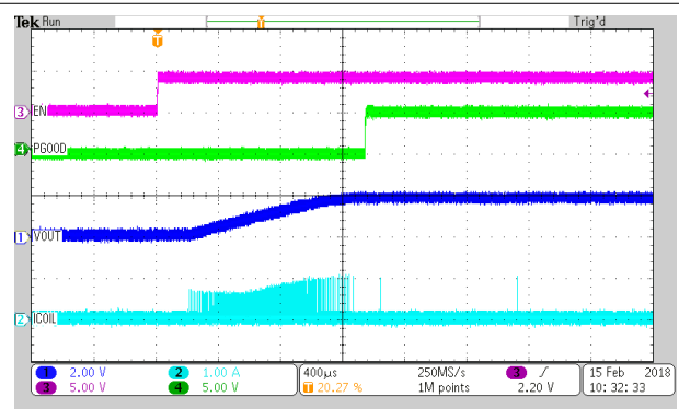
TPS62824/5/6 Figure 8-38. Start-Up With No Load
