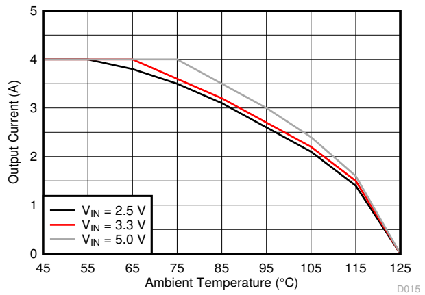
Figure 8-30. Thermal Derating
