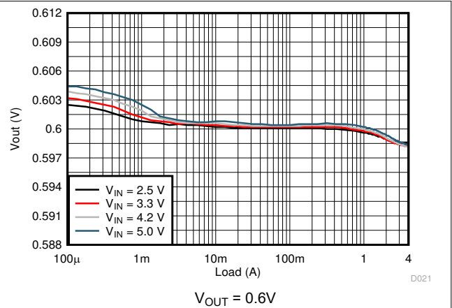
Figure 8-4. Load Regulation
