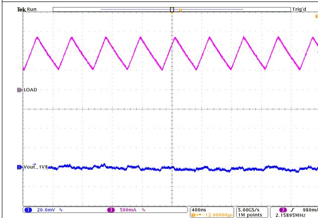
I_{OUT} = 1.0A TPS62824A/5A/6A/7A Figure 8-35. PWM Operation at F-PWM
