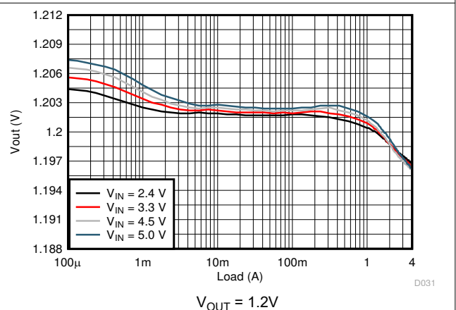
Figure 8-8. Load Regulation
