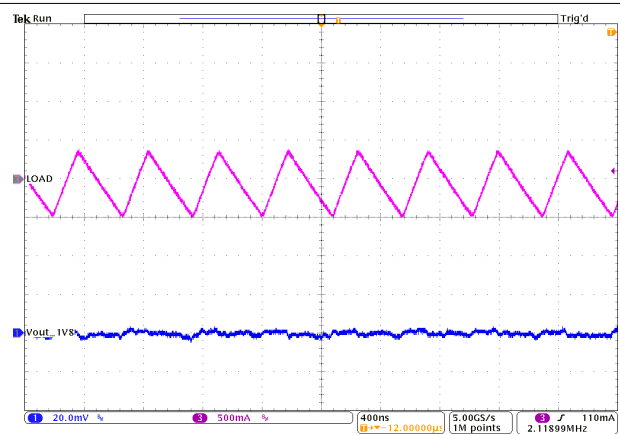
No load TPS62824A/5A/6A/7A Figure 8-36. PWM Operation at F-PWM
