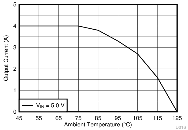
Figure 8-32. Thermal Derating
