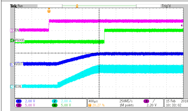
Load = 0.6Ω TPS62826 Figure 8-37. Start-Up With Load
