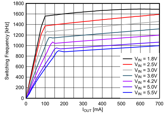
Figure 8-9. Switching Frequency vs Output Current at V_{OUT} = 0.4V
