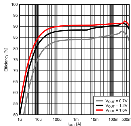
Efficiency vs Output Current at 3.6V VIN
