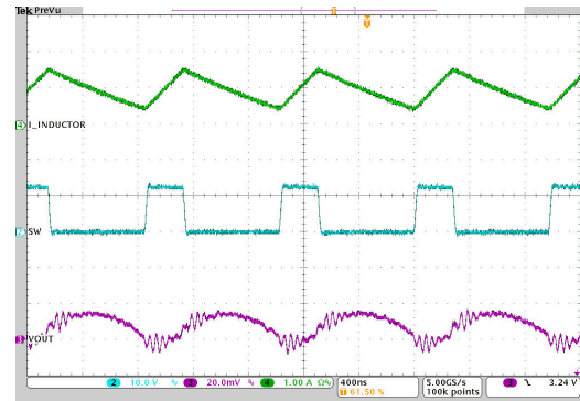
V_{IN} = 12V 1MHz Auto I_o = 1A PFM/PWM V_{OUT} = 3.0V L = 2.2\mu H T_A = 25^\circ C
