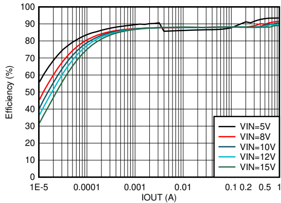
Auto PFM/PWM L = 1µH F sw = 2.5MHz
