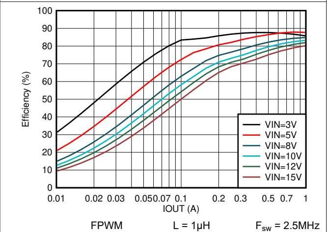
Figure 7-22. Efficiency vs Output Current V OUT = 1.2V
