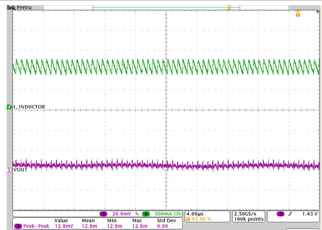
Figure 7-50. Output Voltage Ripple
