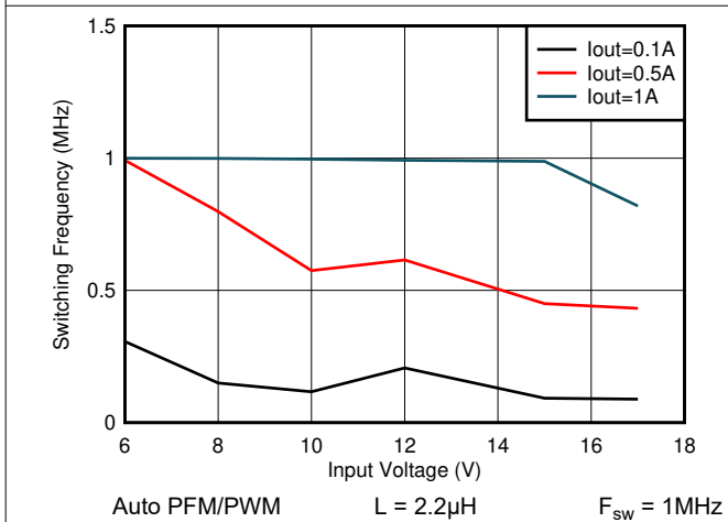
Figure 7-23. Switching Frequency vs Input Voltage V OUT = 5V
