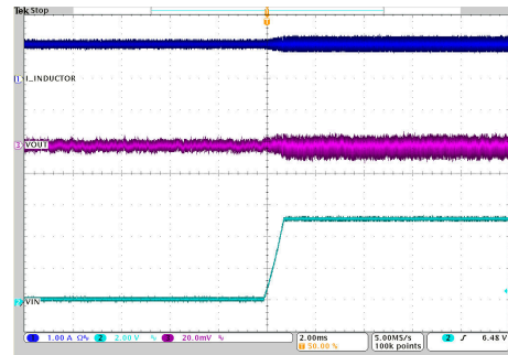
V_{IN} = 6V to 11V 2.5MHz Auto I_o = 1A PFM/PWM
