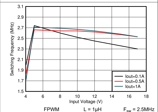
Figure 7-30. Switching Frequency vs Input Voltage V OUT = 3.3V
