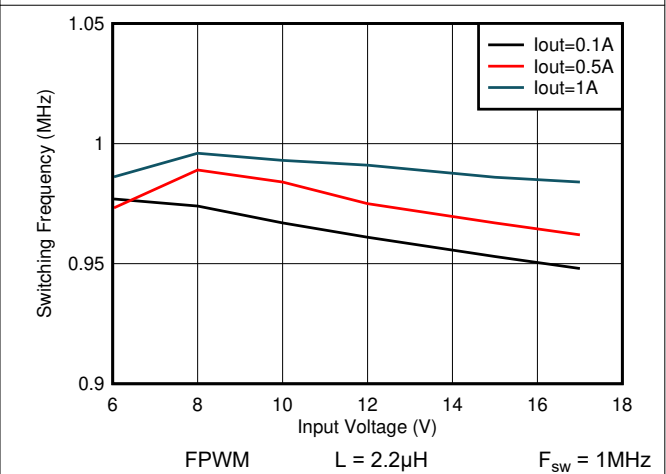
Figure 7-24. Switching Frequency vs Input Voltage V OUT = 5V
