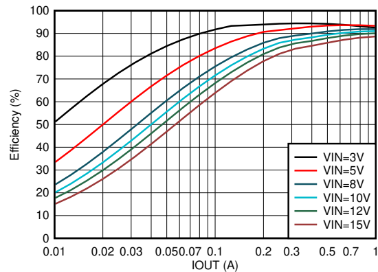
FPWM L = 2.2µH F sw = 1MHz
