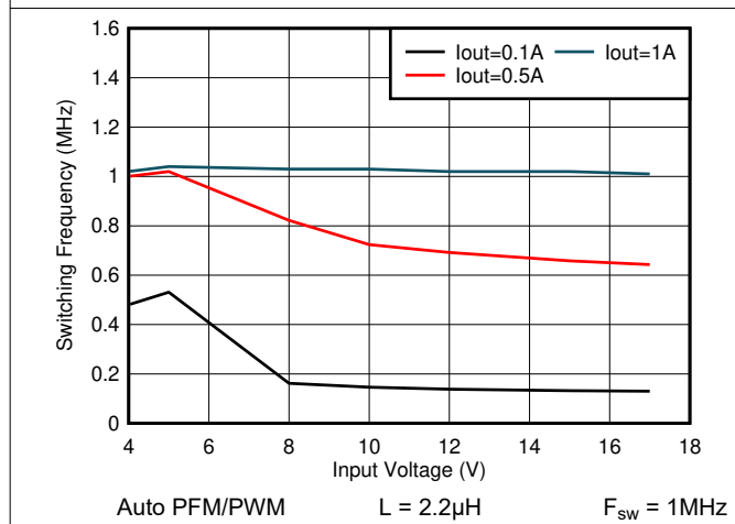
Figure 7-27. Switching Frequency vs Input Voltage V OUT = 3.3V
