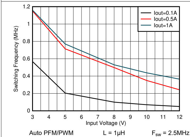
Figure 7-75. Switching Frequency vs Input Voltage V OUT = 0.4V
