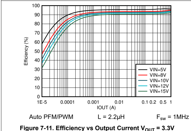
Figure 7-11. Efficiency vs Output Current V_{\text{OUT}} = 3.3\text{V}
