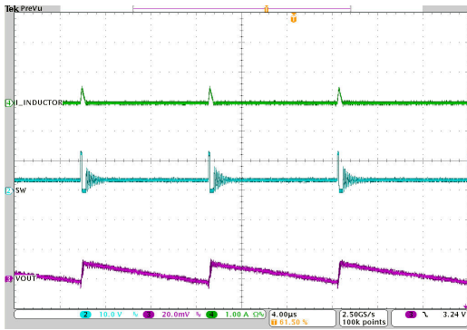
V_{IN} = 12V 2.5MHz Auto I_o = 10mA PFM/PWM V_{OUT} = 3.0V L = 2.2\mu H T_A = 25^\circ C
