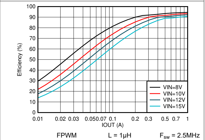
Figure 7-10. Efficiency vs Output Current V_{\text{OUT}} = 5\text{V}
