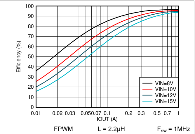
Figure 7-8. Efficiency vs Output Current V_{\text{OUT}} = 5\text{V}
