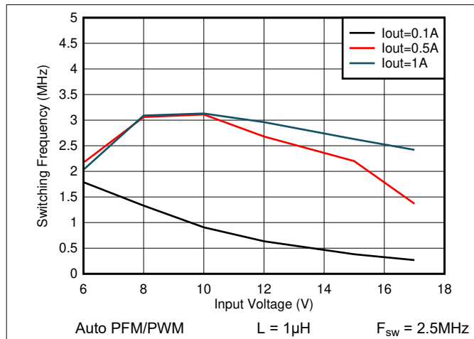
Figure 7-25. Switching Frequency vs Input Voltage V OUT = 5V
