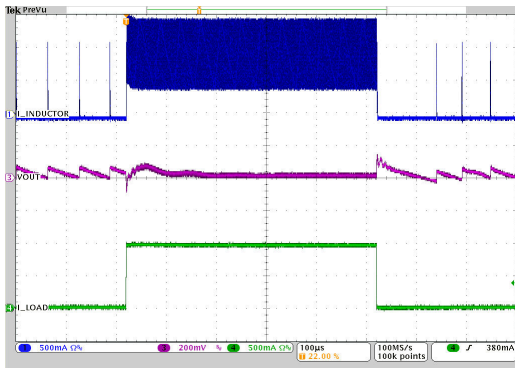
V_{IN} = 12V 1MHz Auto I_o = 5mA to 1A to 5mA PFM/PWM V_{OUT} = 3.3V T_A = 25^\circ C
