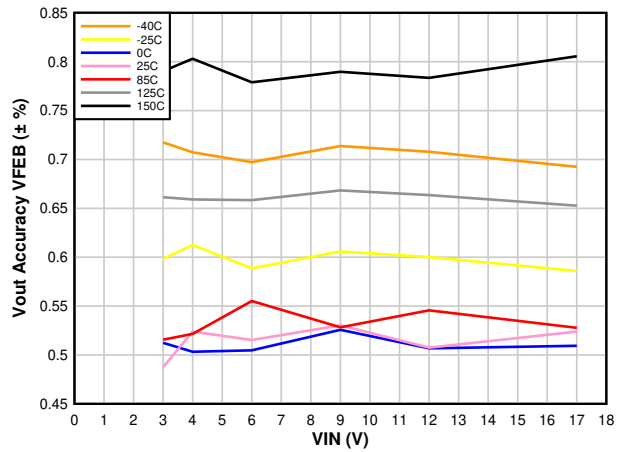
Figure 5-4. Output Voltage Accuracy - VFEB Selected
