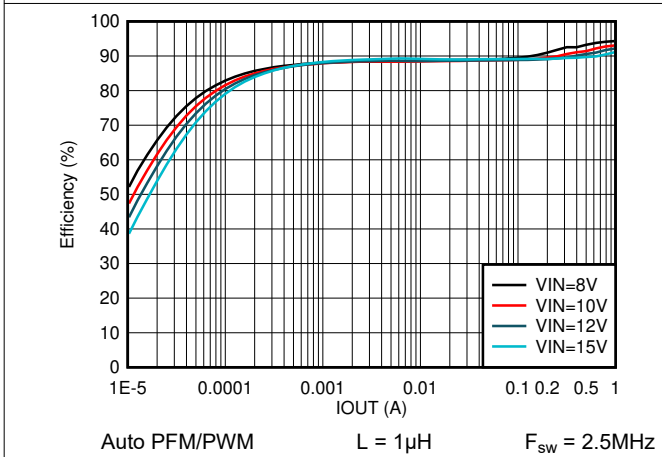
Figure 7-9. Efficiency vs Output Current V_{\text{OUT}} = 5\text{V}
