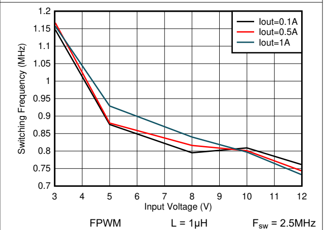
Figure 7-76. Switching Frequency vs Input Voltage V OUT = 0.4V
