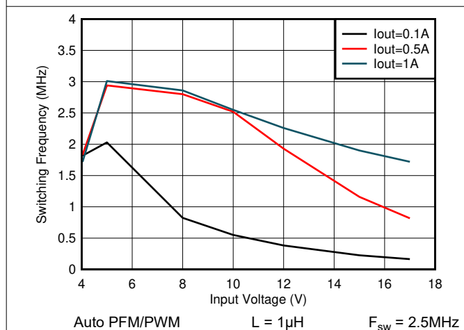
Figure 7-29. Switching Frequency vs Input Voltage V OUT = 3.3V
