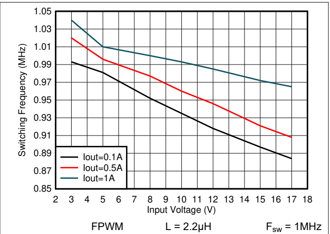
Figure 7-32. Switching Frequency vs Input Voltage V_{OUT} = 1.8V
