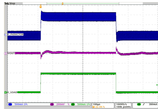
V_{IN} = 12V 2.5MHz FPWM I_o = 5mA to 1A to 5mA V_{OUT} = 3.3V T_A = 25^\circ C
