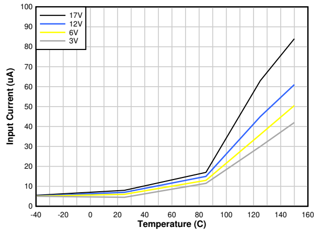
Figure 5-2. Maximum Quiescent Current vs Temperature
