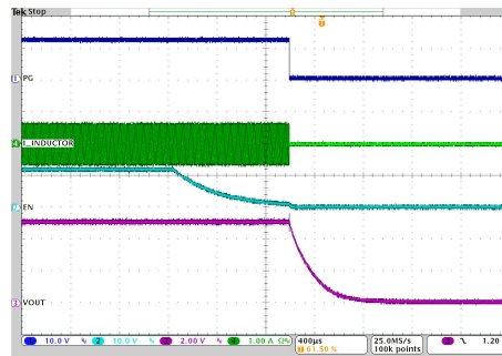
V_{IN} = 12V Output Discharge = Yes V_{OUT} = 5V T_A = 25^\circ C
