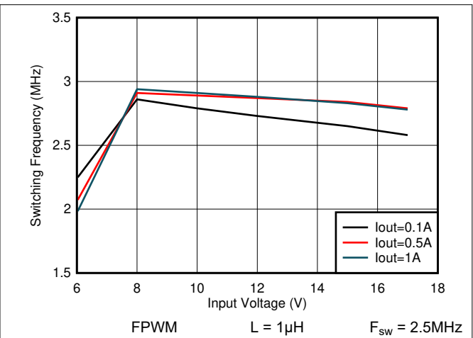
Figure 7-26. Switching Frequency vs Input Voltage V OUT = 5V
