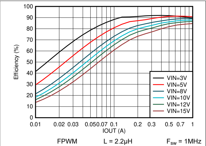
Figure 7-20. Efficiency vs Output Current V OUT = 1.2V
