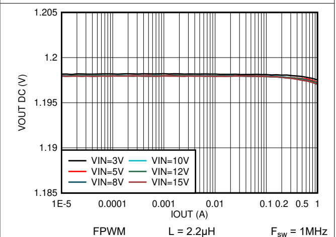
Figure 7-78. Output Voltage vs Output Current V OUT = 1.2V
