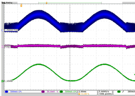
V_{IN} = 12V 1MHz Auto I_o = 0A to 1A PFM/PWM V_{OUT} = 3.3V L = 2.2\mu H T_A = 25^\circ C
