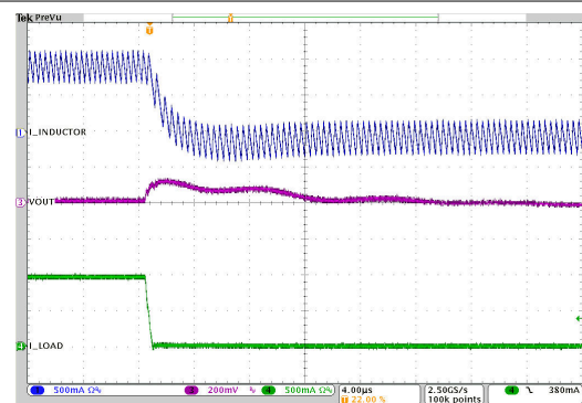
V_{IN} = 12V 2.0MHz FPWM I_o = 1A to 5mA V_{OUT} = 3.3V T_A = 25^\circ C
