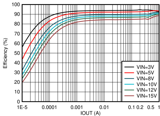
Auto PFM/PWM L = 2.2µH F sw = 1MHz
