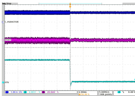
V_{IN} = 11V to 6V 2.5MHz Auto I_o = 1A PFM/PWM
