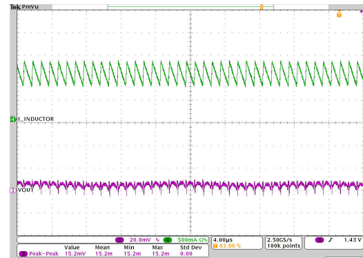
Figure 7-50. Output Voltage Ripple
