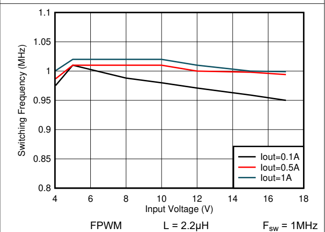
Figure 7-28. Switching Frequency vs Input Voltage V OUT = 3.3V
