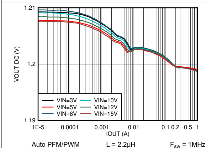
Figure 7-77. Output Voltage vs Output Current V OUT = 1.2V
