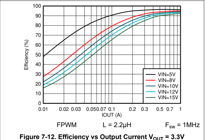
Figure 7-12. Efficiency vs Output Current V_{\text{OUT}} = 3.3\text{V}
