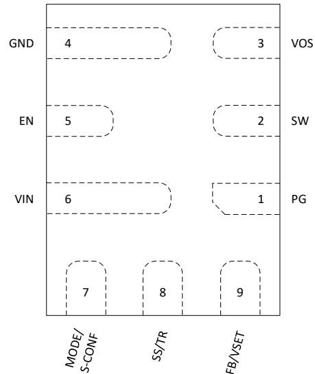
Figure 4-1. 9-Pin RPJ VQFN Package (Top View, Device Pins Face Down)
