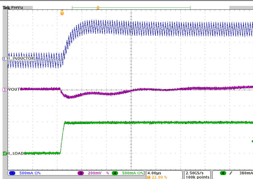
V_{IN} = 12V 2.5MHz FPWM I_o = 5mA to 1A V_{OUT} = 3.3V T_A = 25^\circ C
