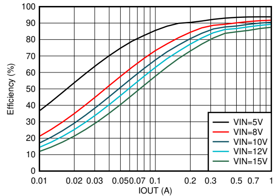
FPWM L = 1µH F sw = 2.5MHz
