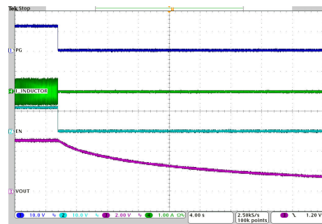
V_{IN} = 12V Output Discharge = No V_{OUT} = 5V T_A = 25^\circ C
