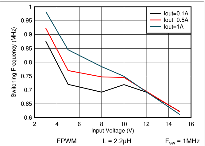
Figure 7-74. Switching Frequency vs Input Voltage V OUT = 0.4V
