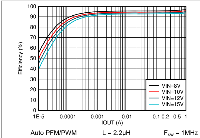
Figure 7-7. Efficiency vs Output Current V_{\text{OUT}} = 5\text{V}
