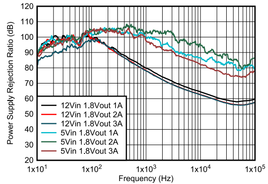
12 V to 1.8 V 2.2 μH, 1 MHz 1 A, 2 A, 3 A After Ferrite Bead
