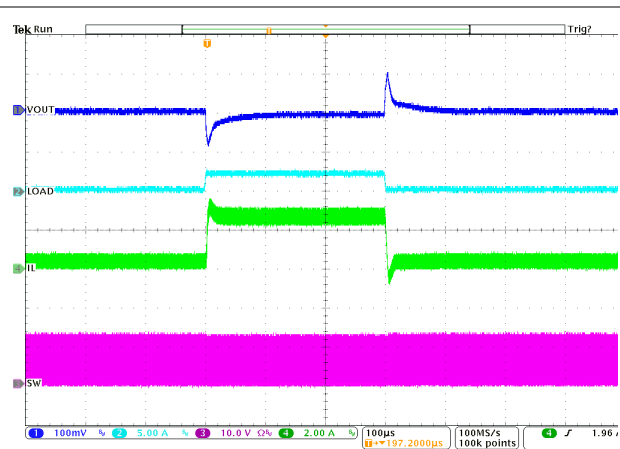
12 V to 1.8 V 2.2 \mu H, 1 MHz After 2nd L-C 300 mA to 2.7 A to 300 mA
