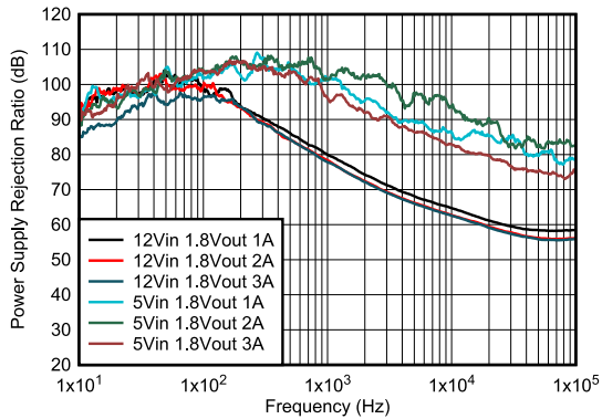
12 V to 1.8 V 2.2 μH, 1 MHz 1 A, 2 A, 3 A First L-C Only, No Ferrite Bead
