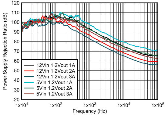
12 V to 1.2 V 2.2 μH, 1 MHz 1 A, 2 A, 3 A First L-C Only, No Ferrite Bead
