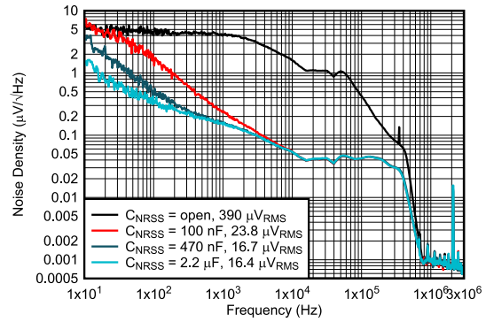
5 V to 3.3 V 2.2 μH, 2.2 MHz After ferrite bead filter NR/SS = Open, 100 nF, 470 nF, 2.2 μF, BW = 100 Hz to 100 kHz
