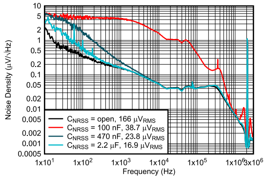
5 V to 3.3 V 2.2 μH, 2.2 MHz First L-C Only NR/SS = Open, 100 nF, 470 nF, 2.2 μF, BW = 100 Hz to 100 kHz
