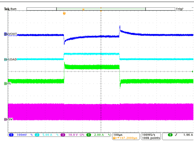
12 V to 3.3 V 2.2 \mu H, 2.2 MHz After 2nd L-C 300 mA to 2.7 A to 300 mA
