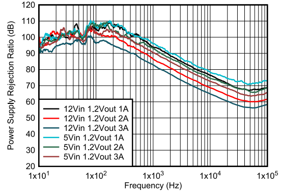
12 V to 1.2 V 2.2 μH, 1 MHz 1 A, 2 A, 3 A After Ferrite Bead Filter
