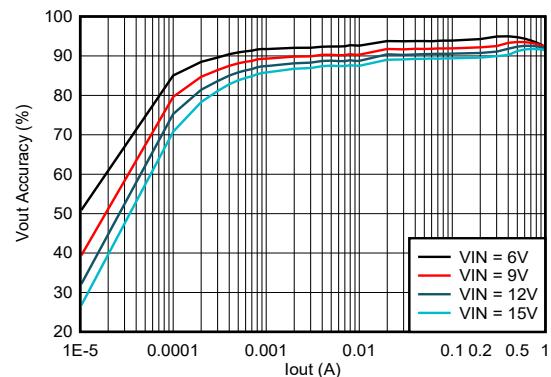
Efficiency vs Output Current V_{OUT} = 3.3 V at 1.0-MHz Auto PFM/PWM
