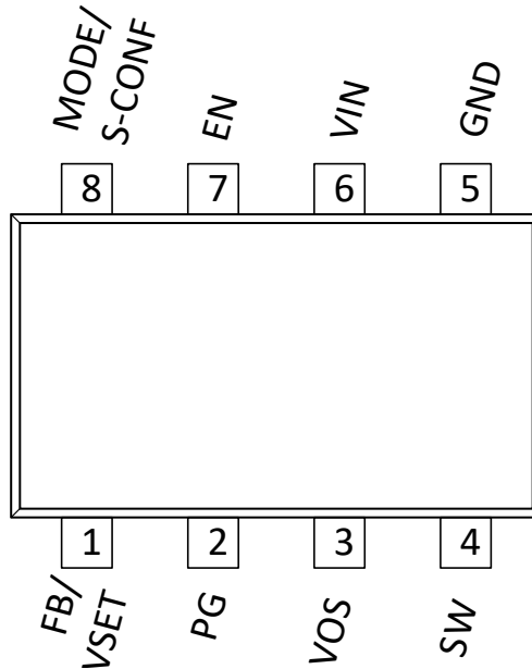
Figure 6-1. TPS629210 Pinout
