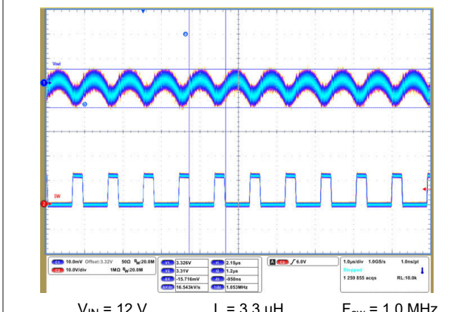
Figure 9-76. Output Voltage Ripple
