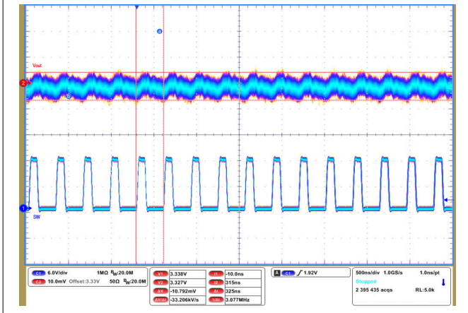
Figure 9-74. Output Voltage Ripple
