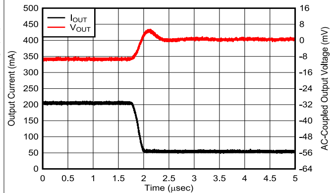
Figure 5-16. Load Transient
