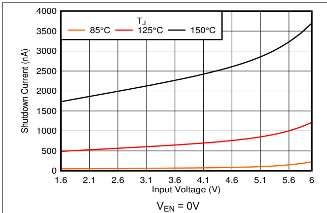
Figure 5-7. Shutdown Current vs V_{IN}
