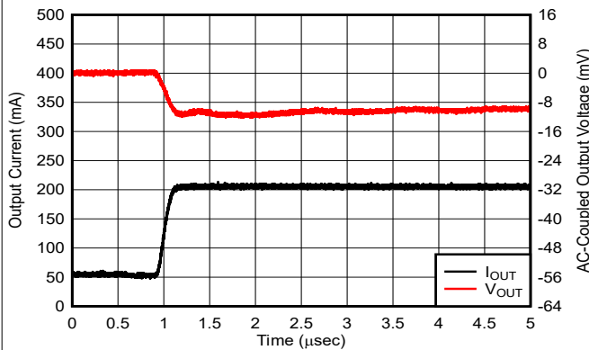
Figure 5-15. Load Transient
