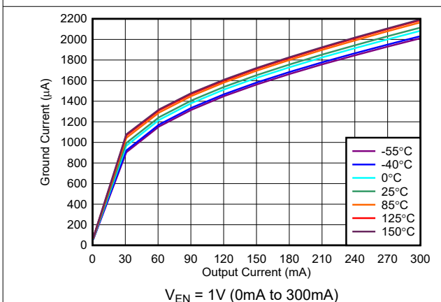
Figure 5-5. I_{GND} vs I_{OUT}
