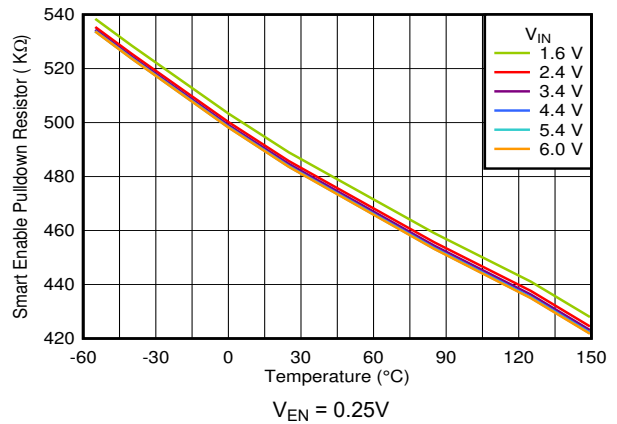
Figure 5-14. Smart Enable Pulldown Resistor vs Temperature and V_{IN}
