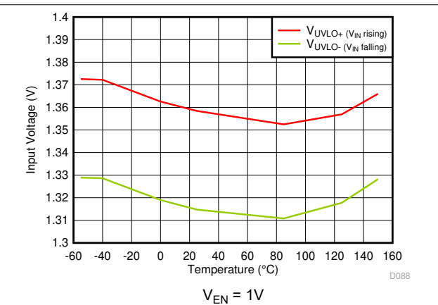
Figure 5-10. UVLO Threshold vs Temperature
