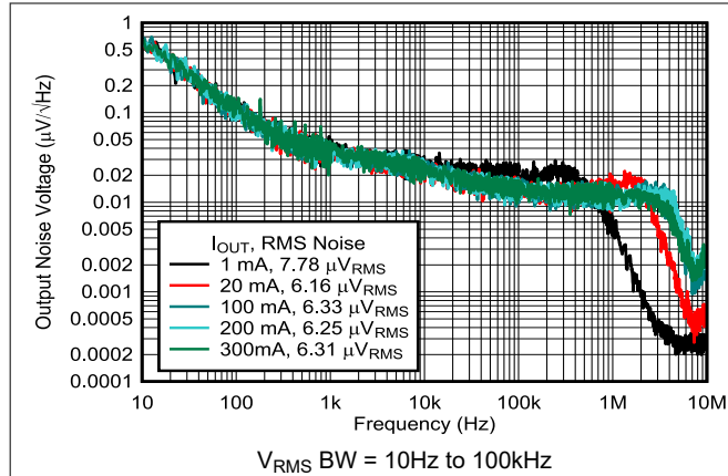
Figure 5-31. Noise vs Frequency and I_{OUT}
