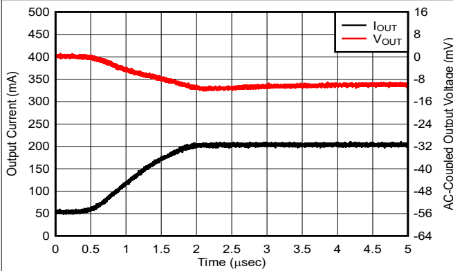
Figure 5-15. Load Transient
