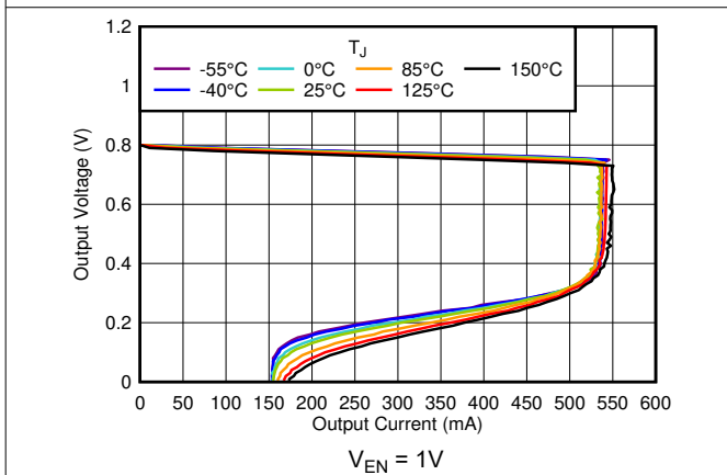
Figure 5-9. Current Limit
