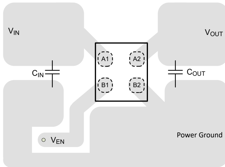
Figure 8-7. Typical DSBGA Layout
