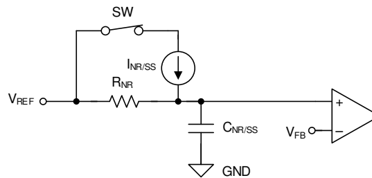
Figure 41. Simplified Soft-Start Circuit
