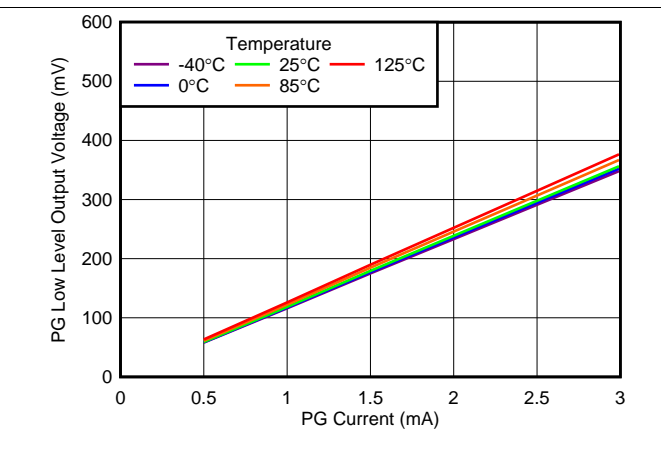
Figure 22. PG Low Level Voltage vs PG Current ( V_{IN} = 6.5\text{ V} )
