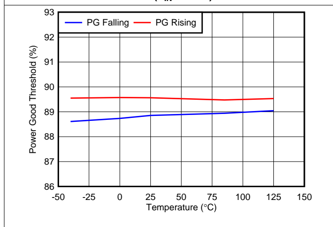
Figure 23. PG Threshold vs Temperature
