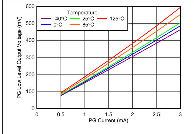
Figure 21. PG Low Level Voltage vs PG Current ( V_{IN} = 1.4\text{ V} )
