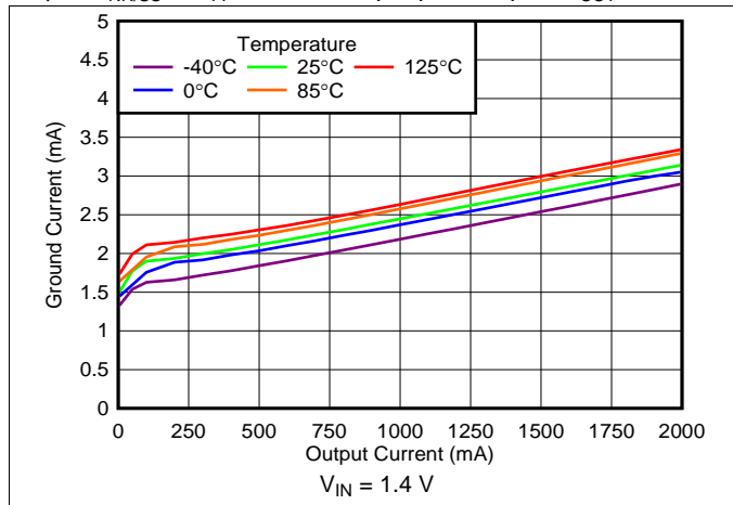
Figure 19. Ground Current vs Output Current
