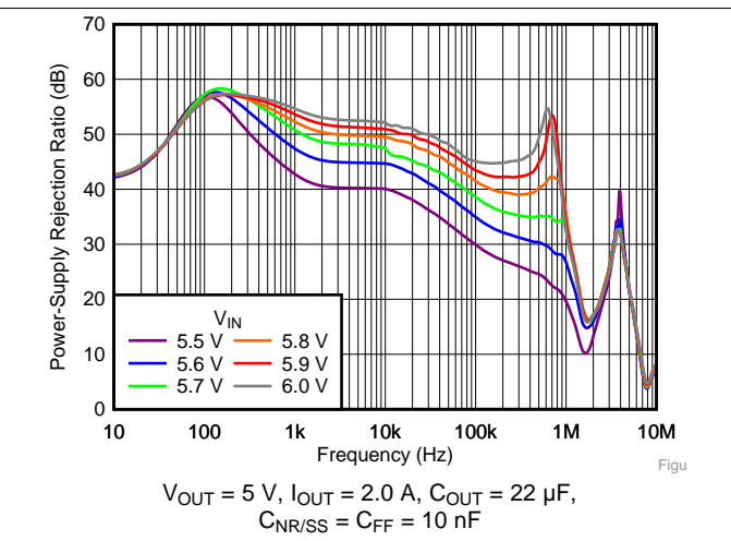
Figure 4. PSRR vs Frequency and Input Voltage
