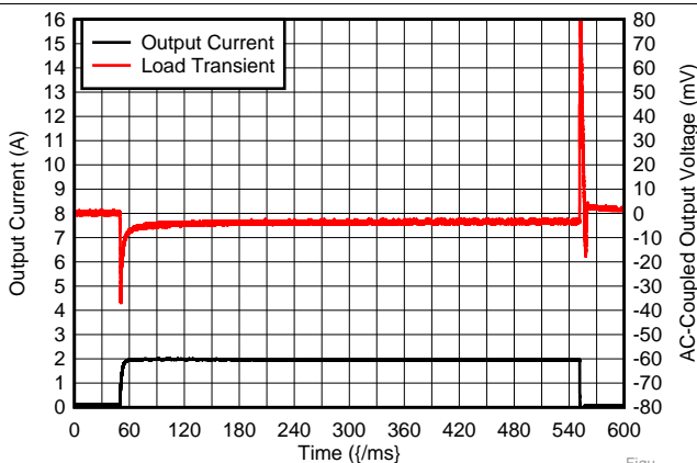
V_{IN} = 1.5\text{ V} , I_{OUT} = 100\text{ mA to } 2\text{ A to } 100\text{ mA at } 1\ \mu\text{s} , C_{OUT} = 22\ \mu\text{F} , V_{PG} = V_{OUT}
