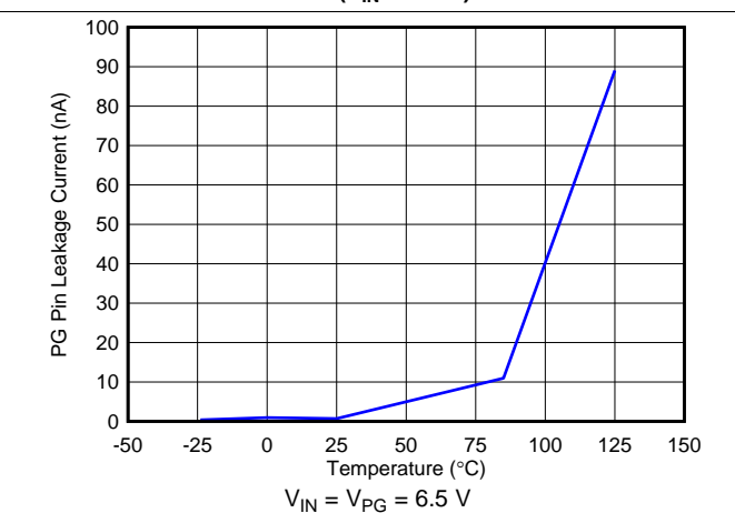
Figure 24. PG Leakage Current vs Temperature
