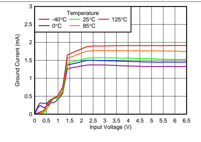
Figure 20. Ground Current vs Input Voltage
