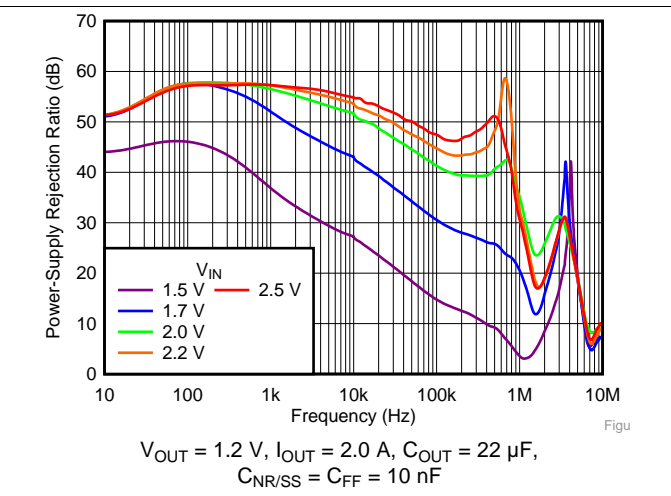
Figure 2. PSRR vs Frequency and Input Voltage
