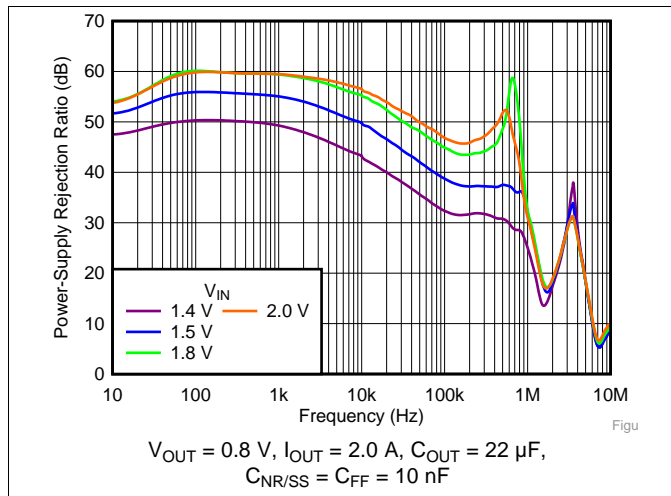
Figure 1. PSRR vs Frequency and Input Voltage
