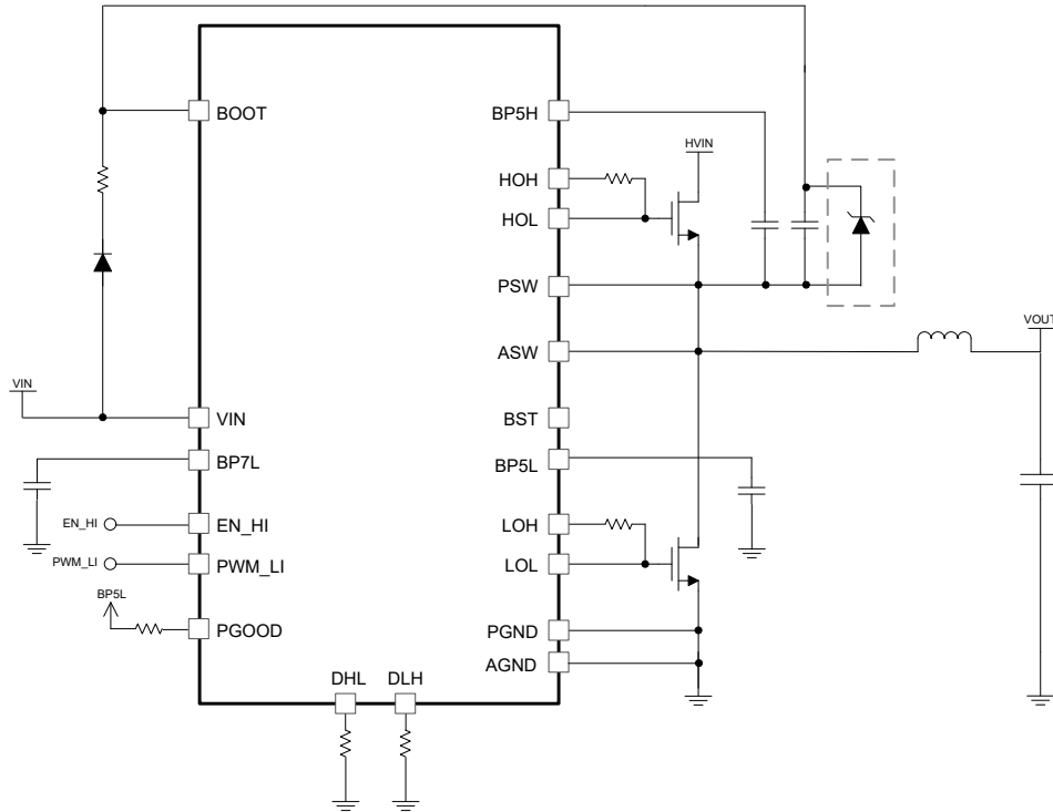
Figure 8-2. Direct VIN Bootstrap Charging Configuration
