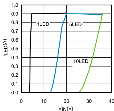
Figure 36. Parallel Operation Results for I_{LED} = 900\text{mA} , I_{LED} vs V_{IN}
