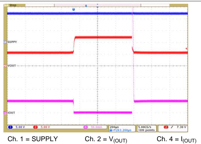
Figure 17. LED Open-Circuit and Recovery
