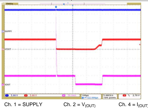
Figure 18. LED Short-Circuit Protection and Recovery
