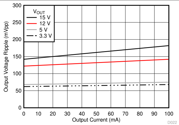
Figure 6-19. Output Voltage Ripple C_{OUT} = 47 \mu\text{F} , 16-V, ceramic
