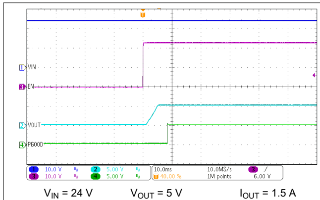
Figure 9-2. Start-up Waveforms
