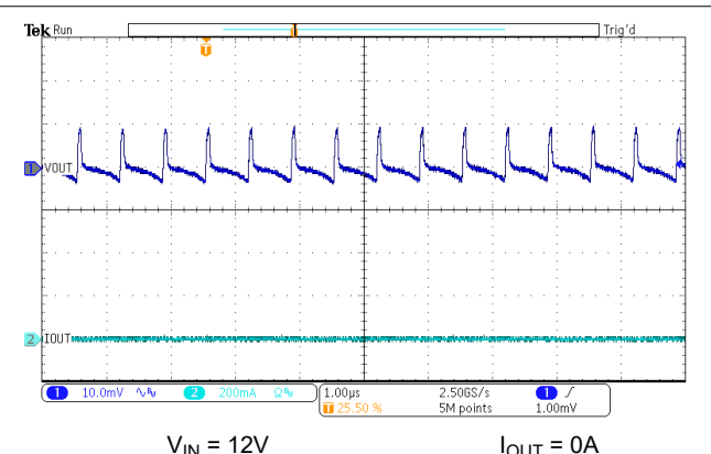
Figure 7-15. Output Ripple – No Load
