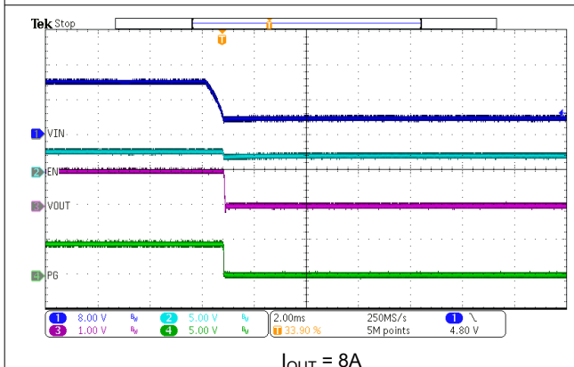
Figure 7-14. VIN Shutdown
