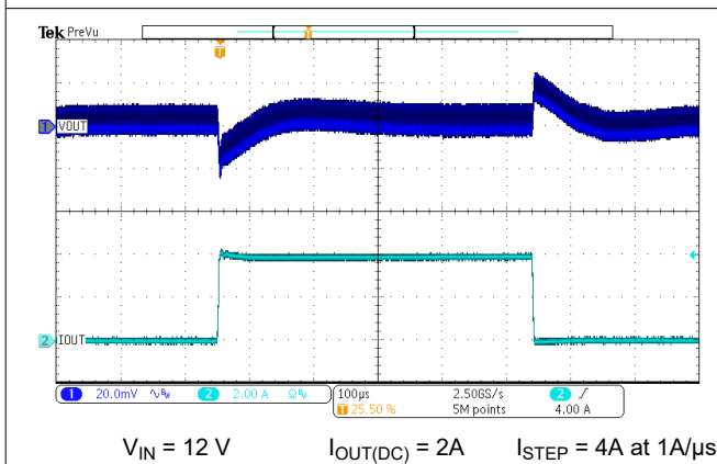
Figure 7-8. Load Transient
