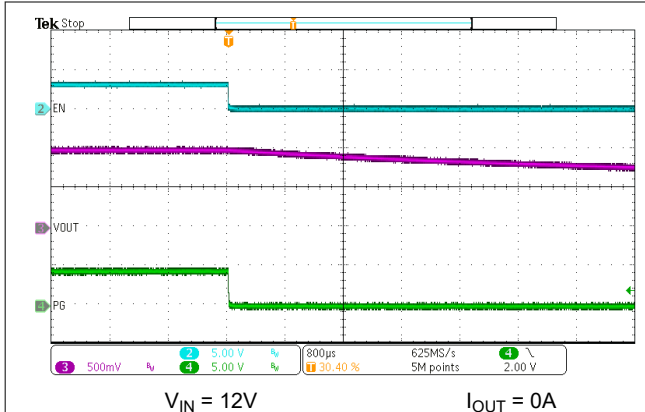
Figure 7-10. EN Shutdown No Load
