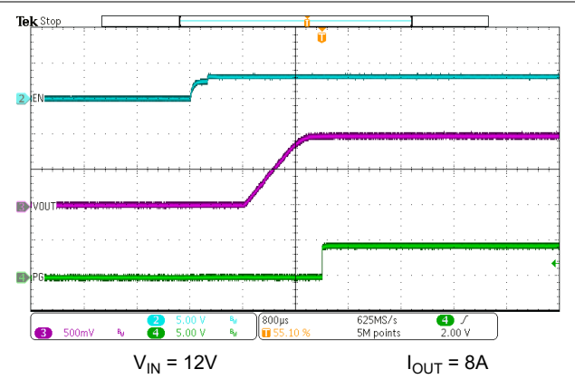
Figure 7-11. EN Start-Up – With Load
