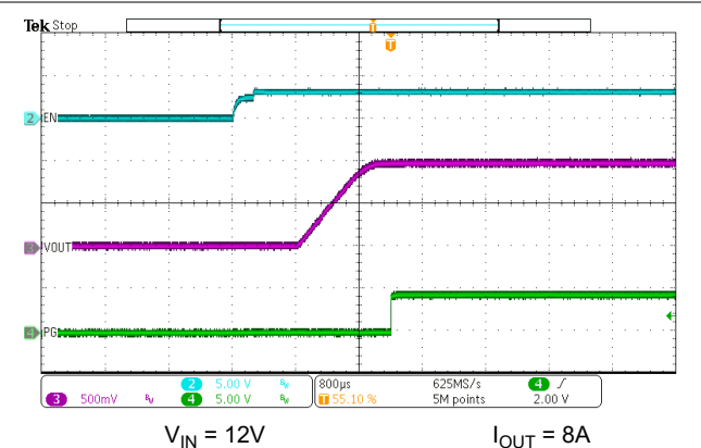
Figure 7-11. EN Start-Up – With Load
