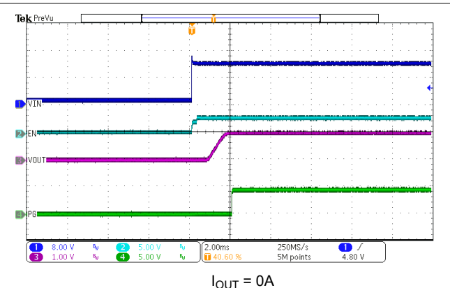
Figure 7-13. VIN Start-Up
