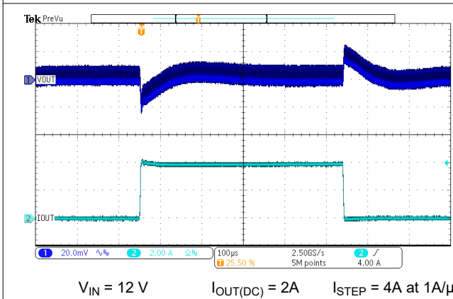
Figure 7-8. Load Transient
