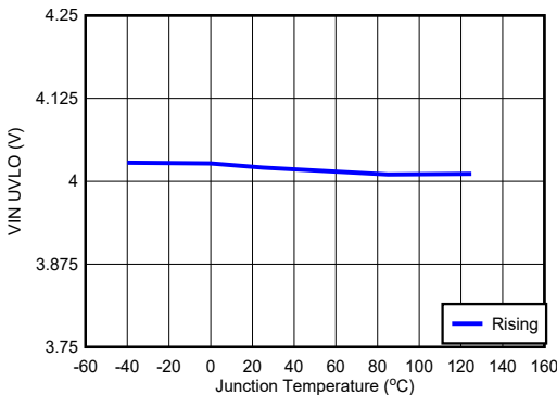
Figure 6-7. V_{IN} UVLO
