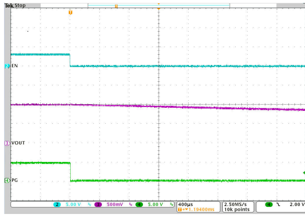
Figure 8-10. EN Shutdown
