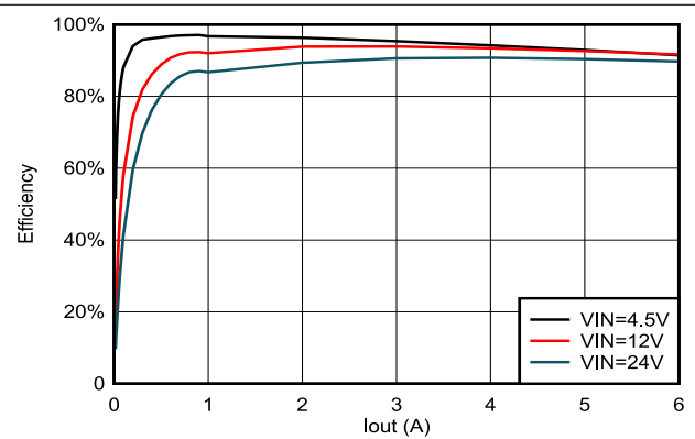
Figure 5-24. TPSM86638 Efficiency, V_{OUT} = 3.3V , F_{sw} = 800kHz
