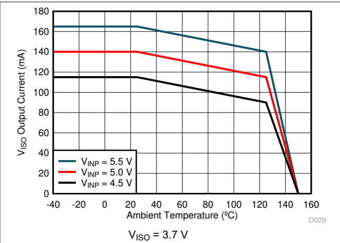
Figure 6-11. Maximum V_{ISO} Output Current vs. Temperature
