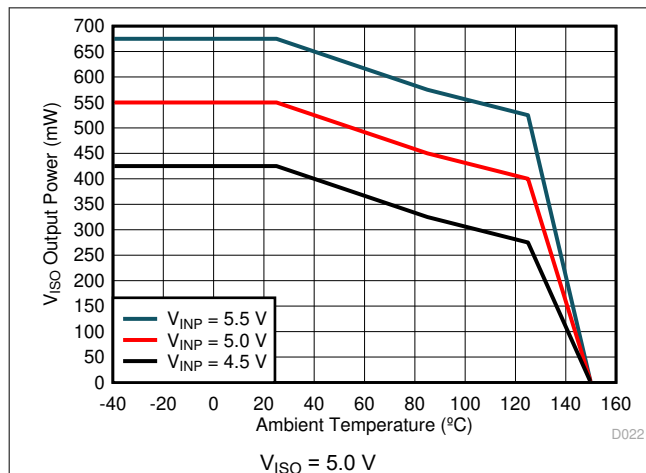
Figure 6-4. Maximum V_{ISO} Output Power vs. Temperature
