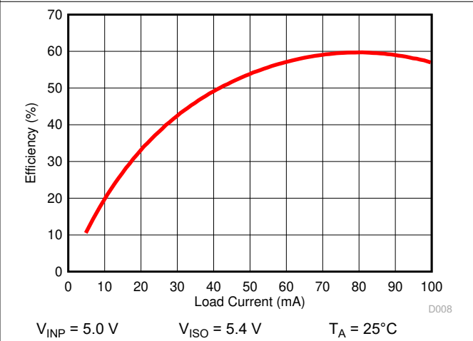
Figure 6-13. Power Supply Efficiency vs. Load Current ( I_{ISO} )
