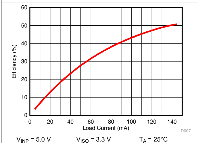
Figure 6-14. Power Supply Efficiency vs. Load Current ( I_{ISO} )
