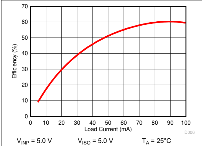
Figure 6-12. Power Supply Efficiency vs. Load Current ( I_{ISO} )
