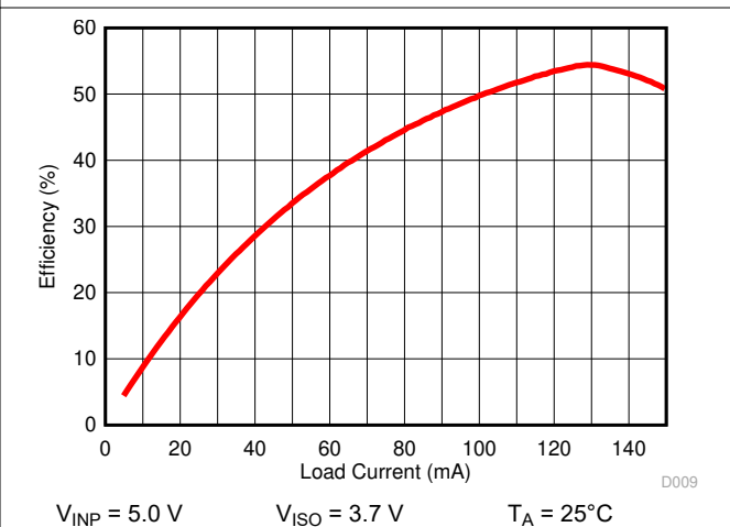
Figure 6-15. Power Supply Efficiency vs. Load Current ( I_{ISO} )
