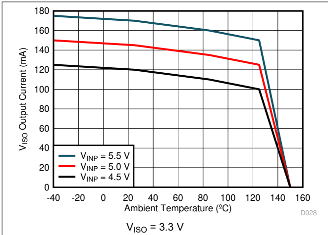
Figure 6-10. Maximum V_{ISO} Output Current vs. Temperature
