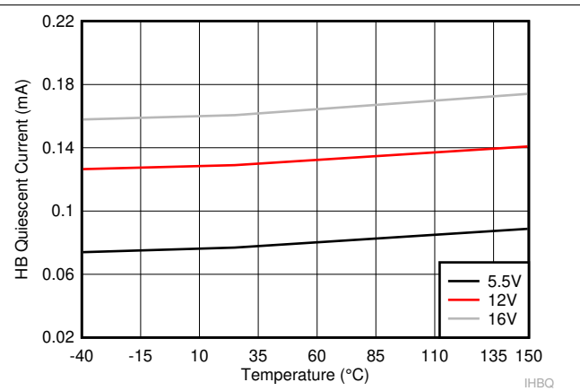
A. V_{HI} = V_{LI} = 0\text{ V} Figure 6-2. HB Quiescent Current
