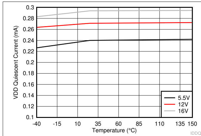
A. V_{HI} = V_{LI} = 0\text{ V} Figure 6-1. VDD Quiescent Current
