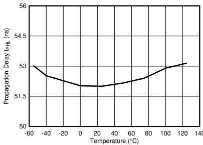
Figure 5-15. Propagation Delay t_{PHL} vs Temperature
