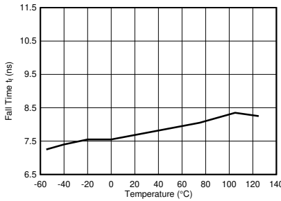
Figure 5-13. Fall Time vs Temperature
