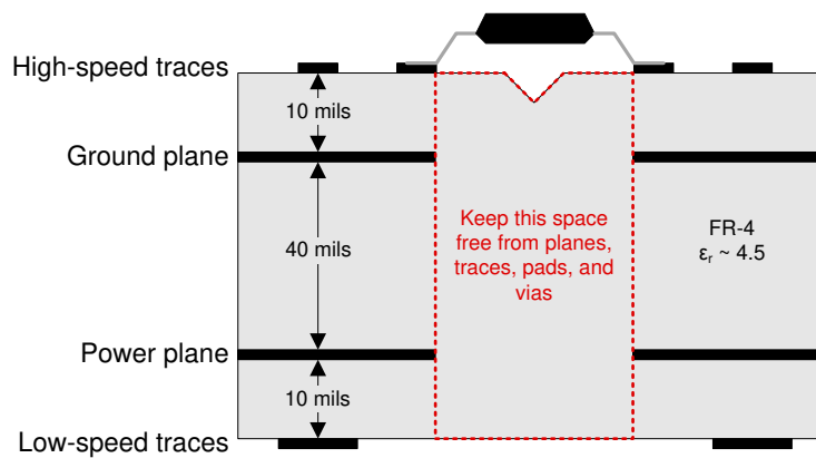
Figure 10-5. Recommended Layer Stack
