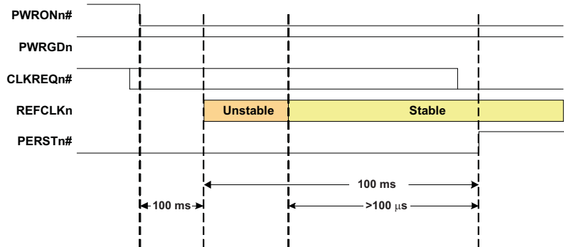
Figure 5-3. PCI Hot Plug Power-Up Cycle With No PWGRDn Feedback
