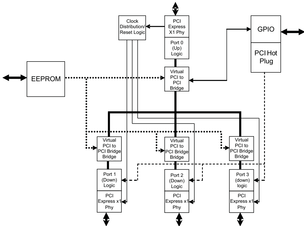
Figure 3-1. Block Diagram
