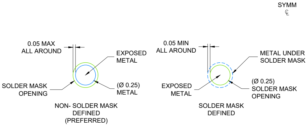
SOLDER MASK DETAILS NOT TO SCALE
