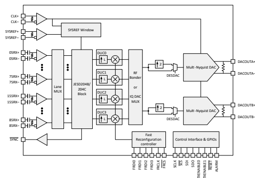
Block Diagram
