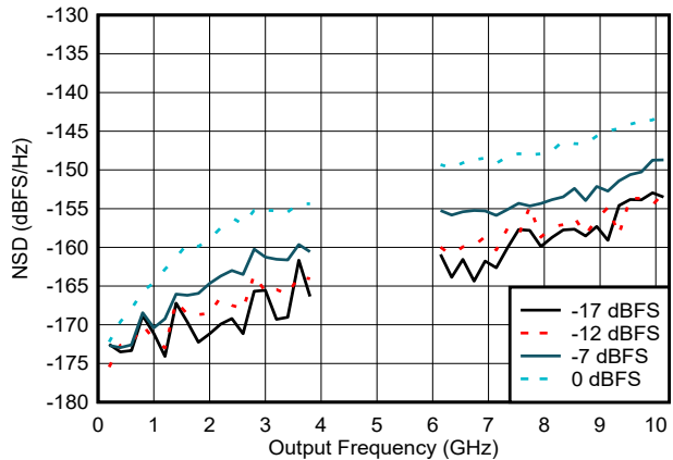
Figure 6-70. NSD vs Output Frequency and Digital Amplitude
