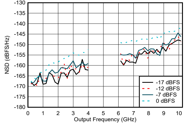
Figure 6-71. NSD vs Output Frequency and Digital Amplitude
