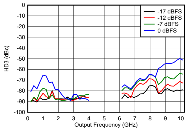
Figure 6-164. HD3 vs Frequency and Digital Amplitude in NRZ/RF Modes
