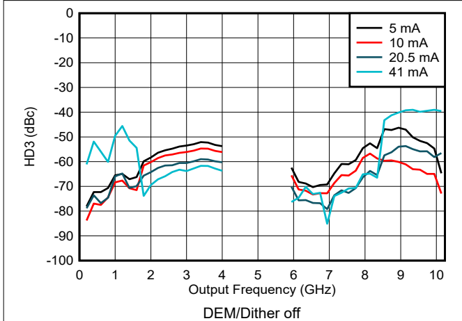
Figure 6-159. HD3 vs Frequency and Output Current in DES2X Modes
