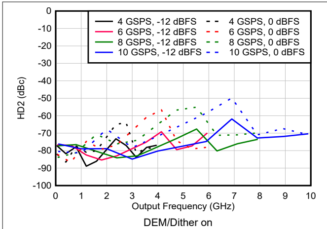
Figure 6-155. HD2 vs Frequency and Sample Rate in DES2X Modes
