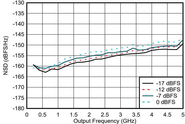
Figure 6-70. NSD vs Output Frequency and Digital Amplitude
