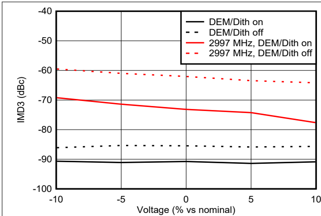
Figure 6-137. IMD3 vs Voltage in NRZ Mode
