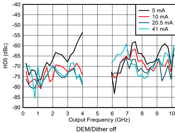
Figure 6-179. HD5 vs Frequency and Output Current in DES2X Modes
