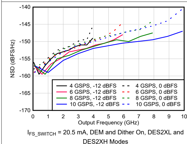
Figure 6-80. NSD vs Output Frequency and Sample Rate
