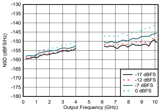
Figure 6-72. NSD vs Output Frequency and Digital Amplitude
