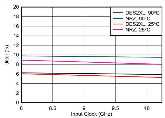
Figure 6-206. Jitter vs Input Clock
