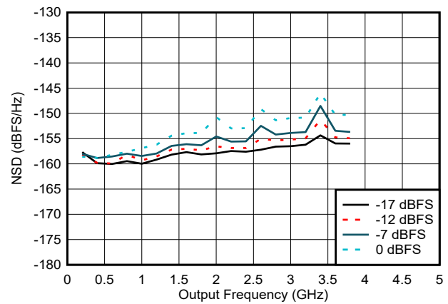
Figure 6-73. NSD vs Output Frequency and Digital Amplitude
