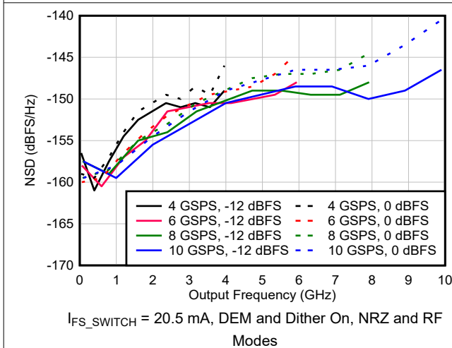
Figure 6-78. NSD vs Output Frequency and Sample Rate
